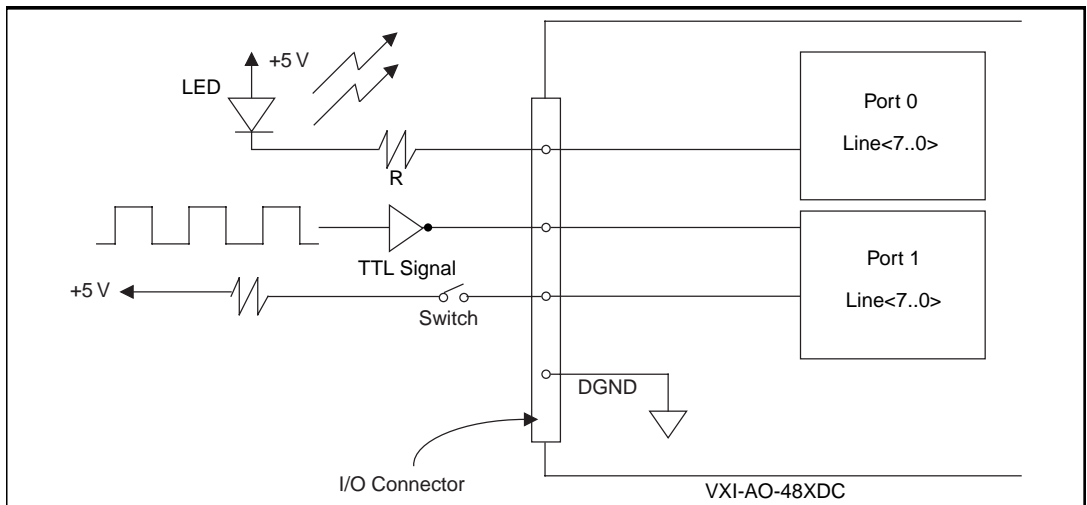
Figure 3-5. Digital I/O Connections
