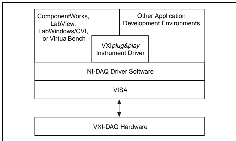
Figure 1-1. The Relationship between the Programming Environment, Your Instrument Driver, and Your VXI-DAQ Hardware
