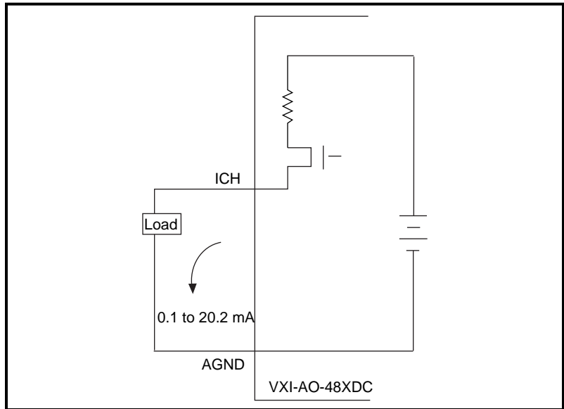
Figure 3-4. ICH Connection as a Current Output
