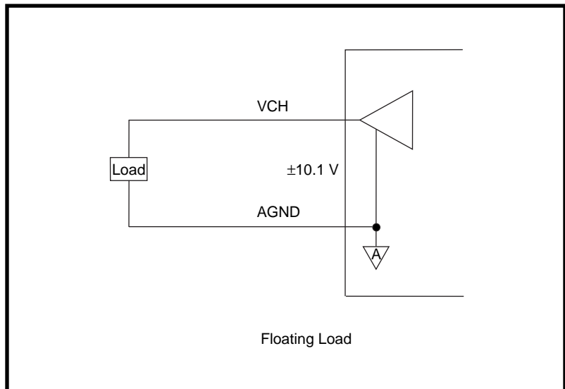
Figure 3-3. VCH Connection as a Voltage Output
